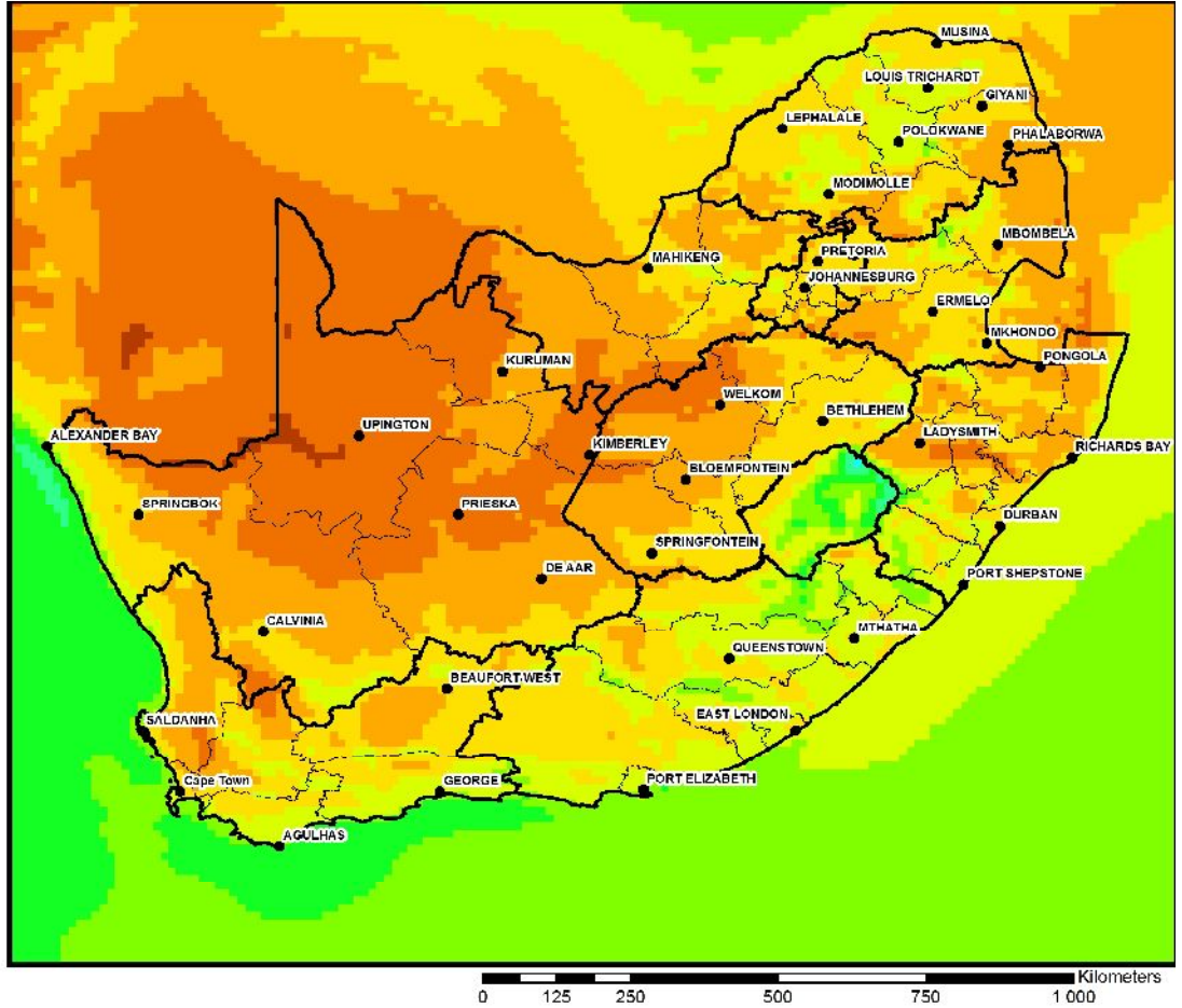
Figure 3: Average Maximum Temperatures 27 March 2018 to 2 April 2018
