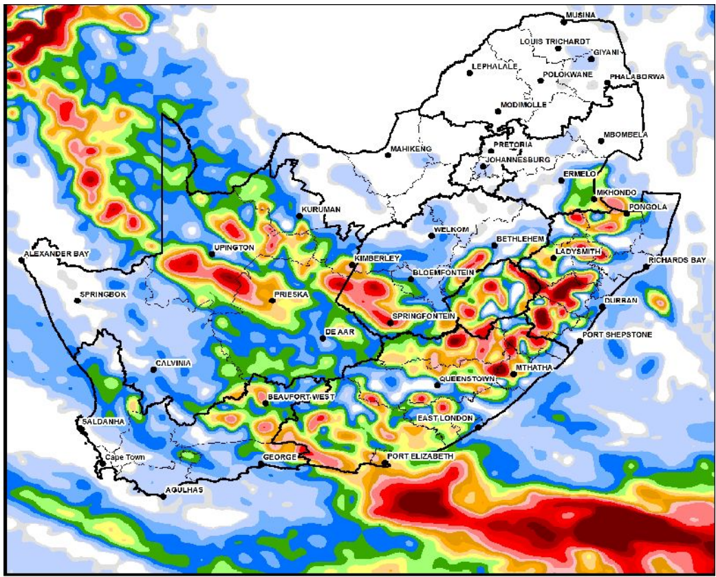
Figure 1: Expected precipitation 27 March 2018 to 2 April 2018.
